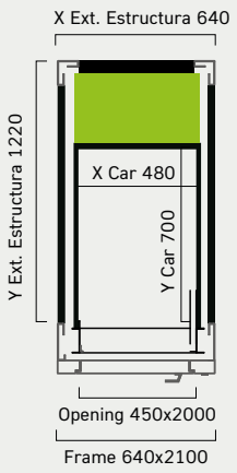
FOLDING DOOR Minimun headroom 2600m
