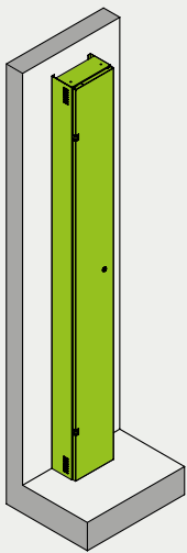
ON THE WALL W280 x D200 x H2100 1 W280 x D200 x H2238 2 Finishes: ✓ As per landing door ✓ If painted metal shaft: the same colour of the shaft
