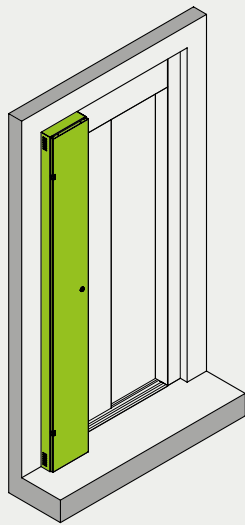
AUTOMATIC DOOR SIDE 1 W280 x D200 x H2238 Finishes: ✓ As per landing door
