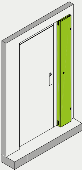
SWING DOOR SIDE 1 W280 x D200 x H2100 Finishes: ✓ As per landing door
