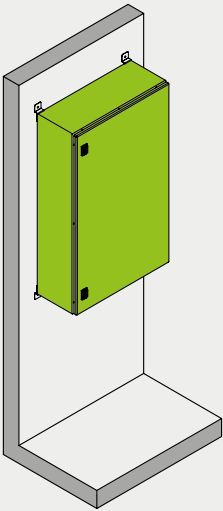
ON THE WALL W600 x D260 x H1000 Finishes: ✓ RAL paint 7035
