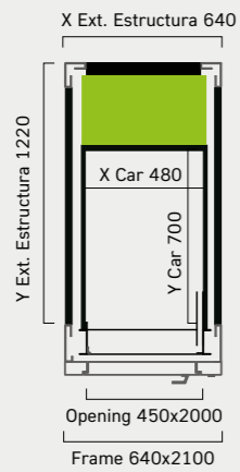
FOLDING DOOR Minimum headroom 2600m
