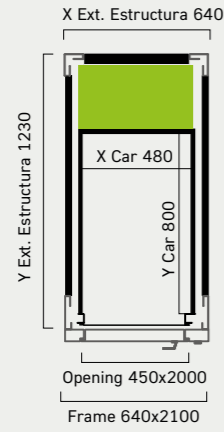
NO DOOR Minimum headroom 2600m
