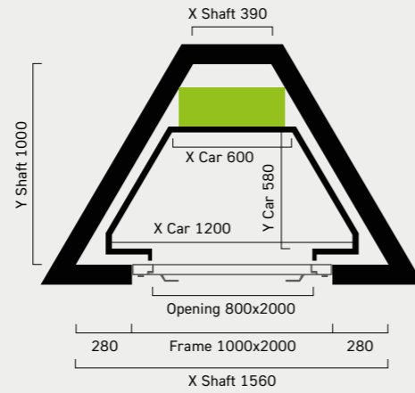
TRAPEZOIDALE Minimum headroom 2600m
