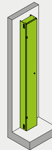
ON THE WALL W280 x D200 x H2100 1 W280 x D200 x H2238 2 Finishes: ✓ As per landing door ✓ If painted metal shaft: the same colour of the shaft
