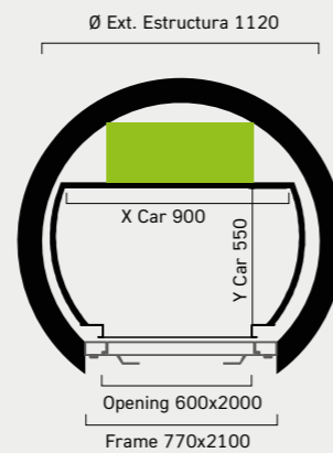
ROUND Minimum headroom 2600m
